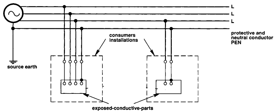
Fig A-3 – TN-C system
