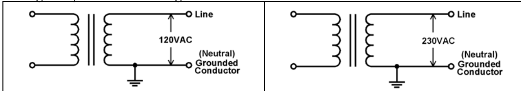
Fig 2 – Single Phase systems
